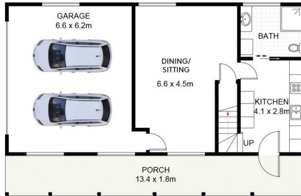
FLOOR 2
