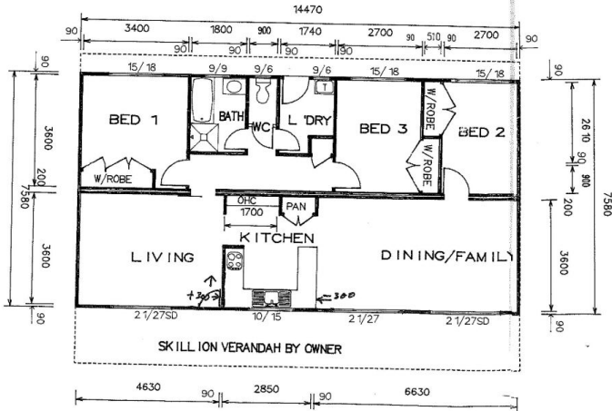
FLOOR PLAN
