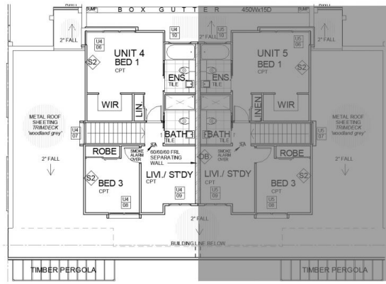
UPPER FLOOR 1:100 @ A1
