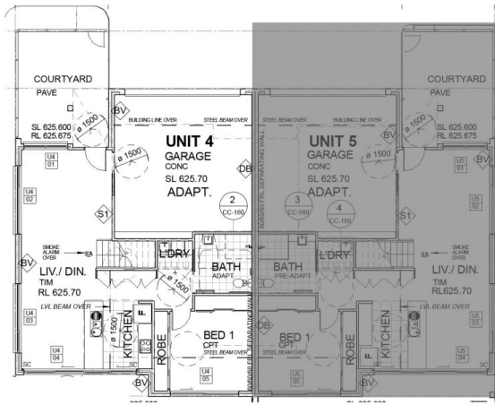
GROUND FLOOR 1:100 @ A1
